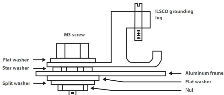
For module with \Phi 4\text{mm} grounding holes
